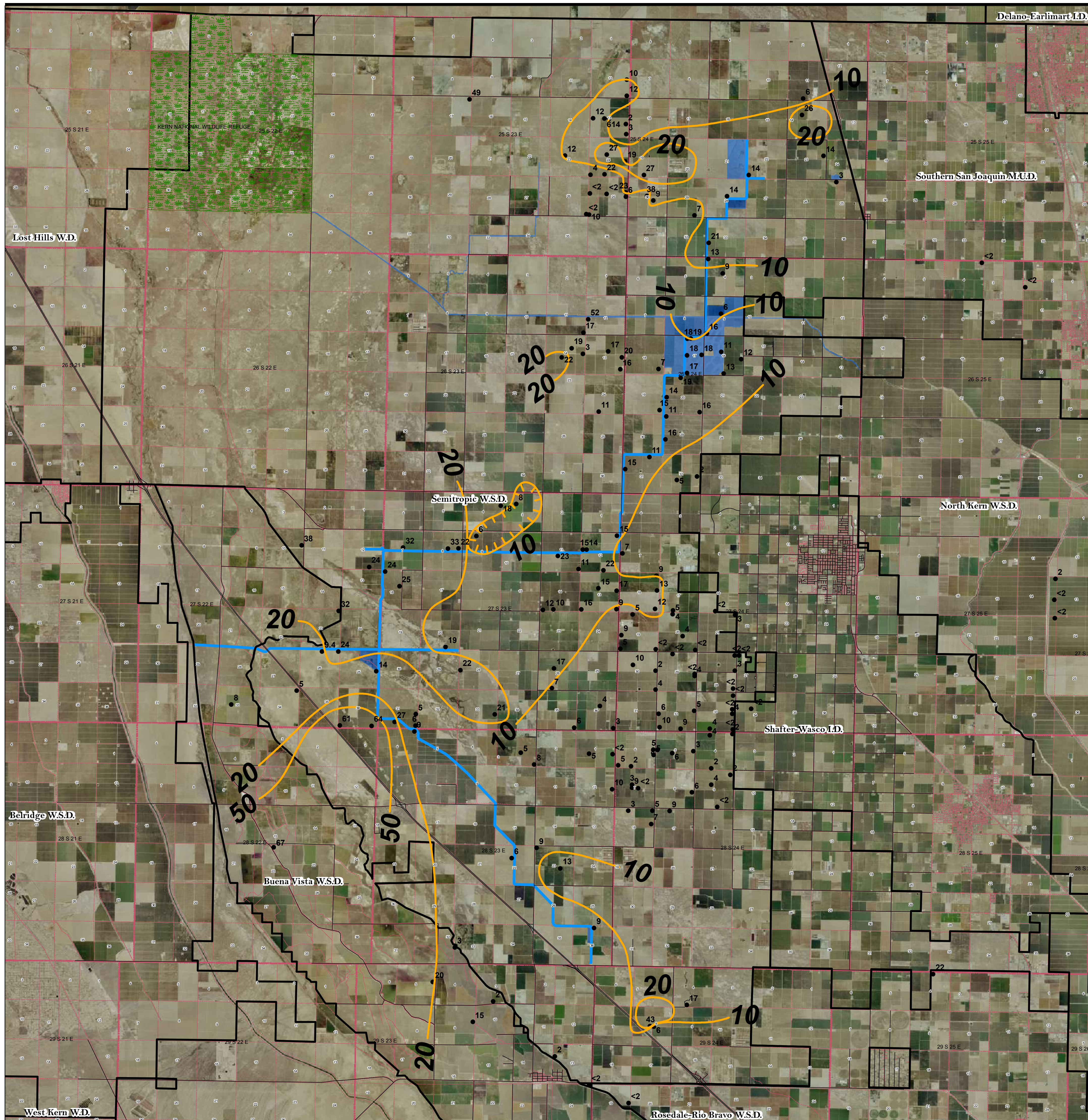
Figure 18 Arsenic Concentrations in Groundwater (March - November 2007)
